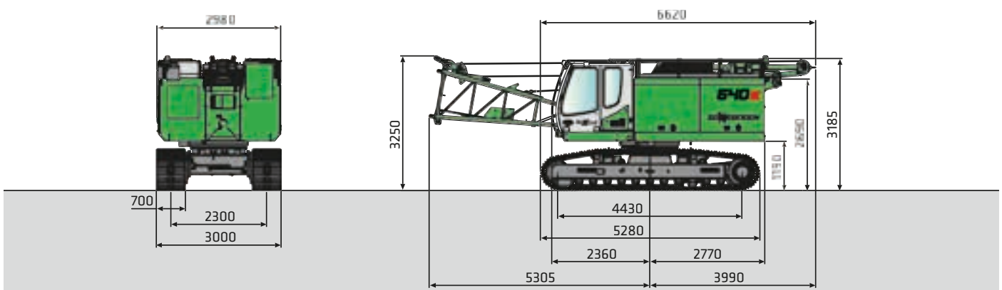
640 HD without counterweight, lower boom section 2 x 12 t freefall winch, approx. 30,500 kg
