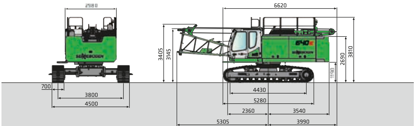
640 HD with counterweight 8.2 t, telescopic undercarriage T41/380, lower boom section 2 x 12 t freefall winch approx 38,700 kg
