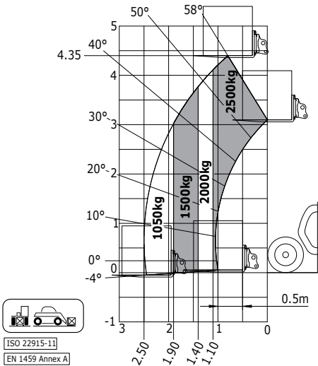
MT 425 H Appendix A industrial
