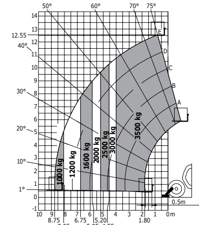
MT 1335/1335 Easy on stabilizers
